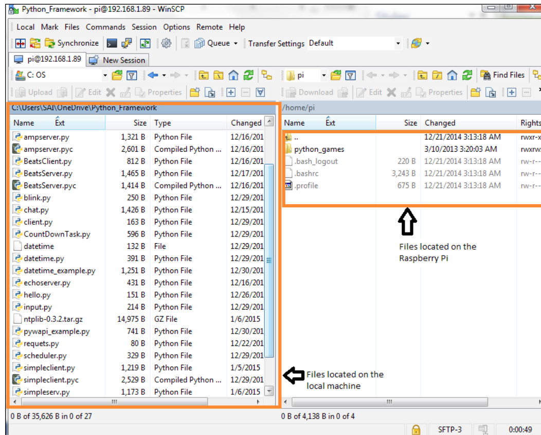
Transferring files using WinSCP
