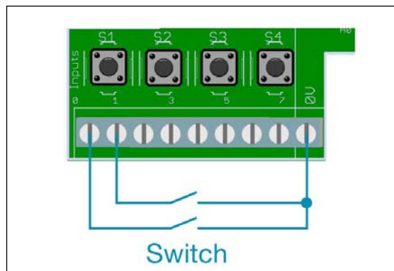
Suggested input connections provided by the PiFace manual
