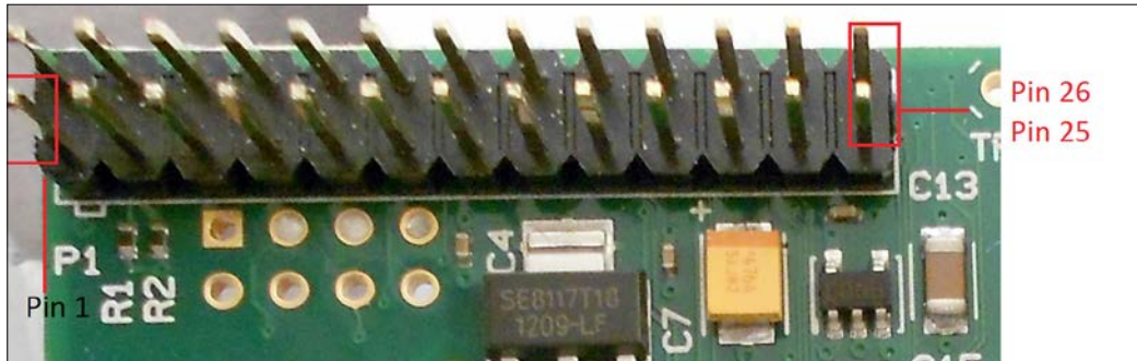
The Raspberry Pi GPIO peripheral
