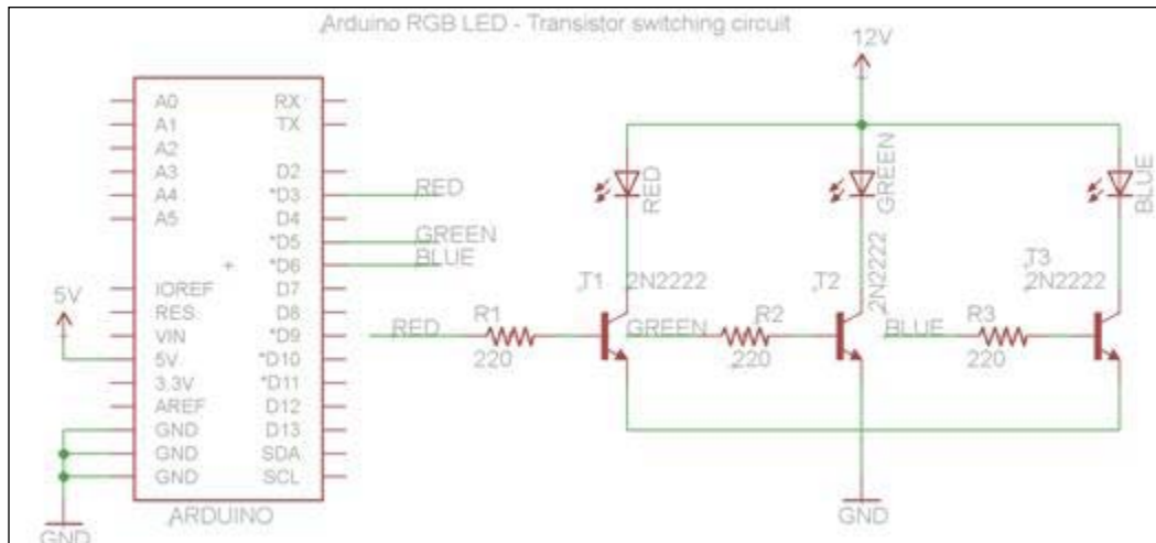
The Arduino RGB switching circuit
