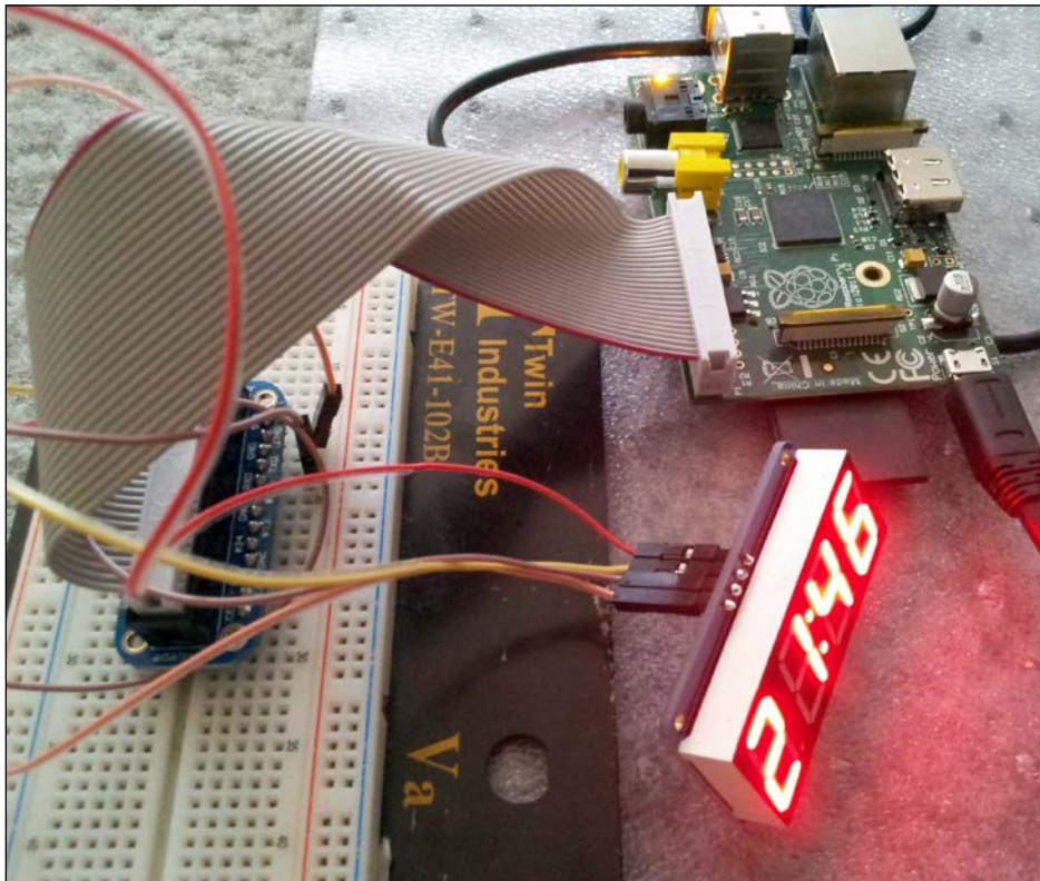
A 7-segment backpack connected to the Cobbler
