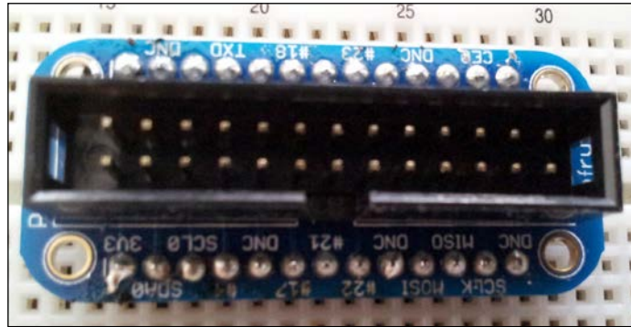
The Cobbler mounted on a breadboard
