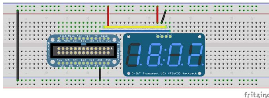
7-segment backpack connections on a breadboard
