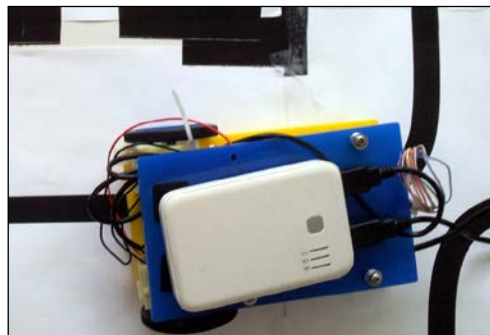
A line following robot
