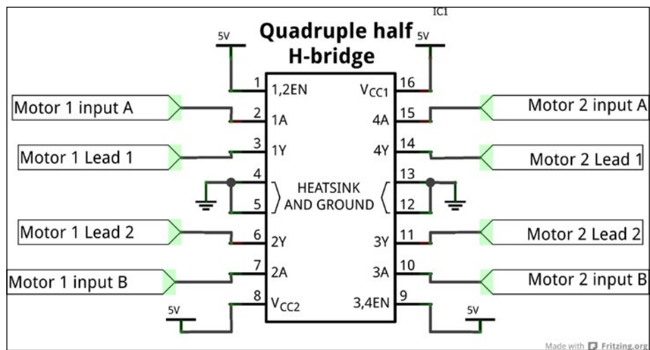
A SN754410 motor control circuitry
