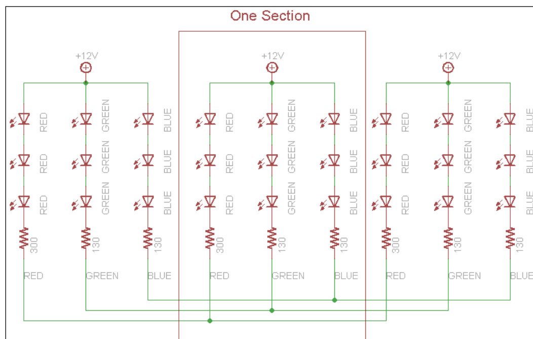
RGB LED strip schematic (borrowed from Adafruit)
