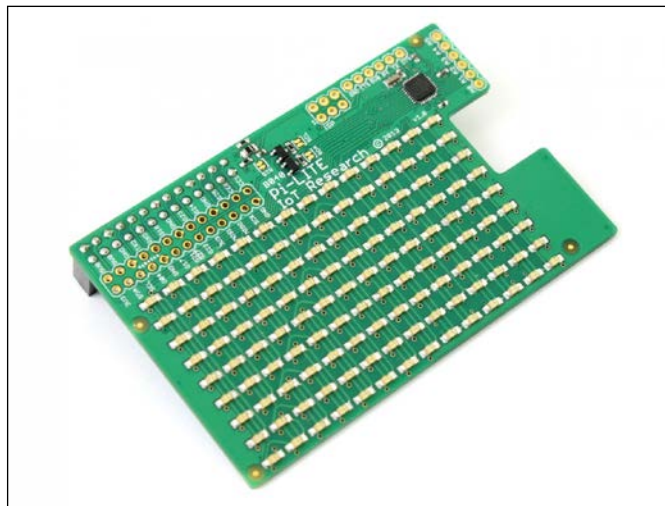
Pi Lite – Courtesy: The Ciseco PLC website
