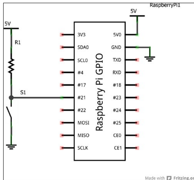
Reed switch setup with the Raspberry Pi GPIO
