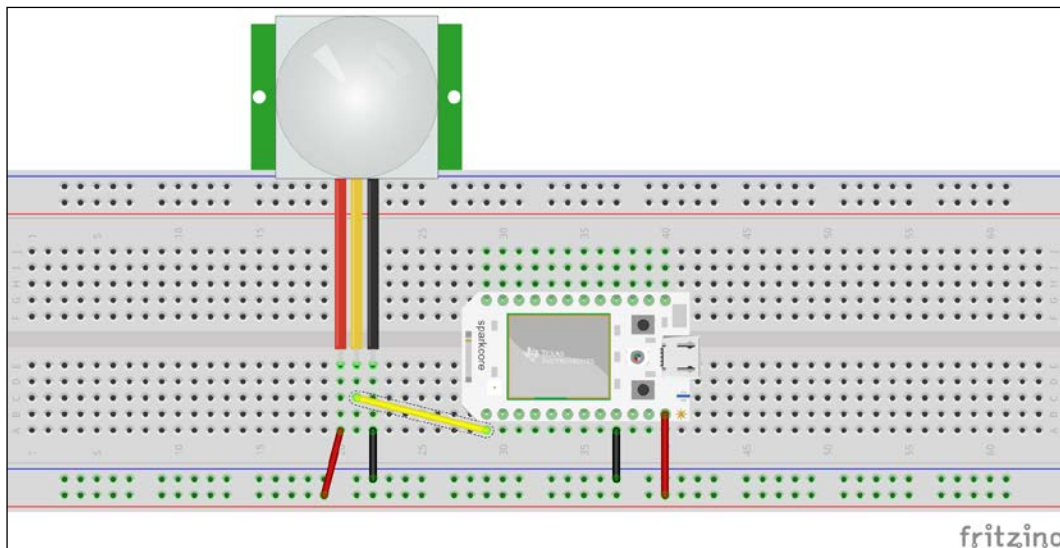
A motion sensor connected to Spark Core
