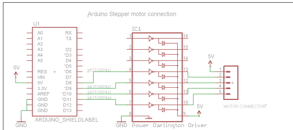
An Arduino stepper motor interface
