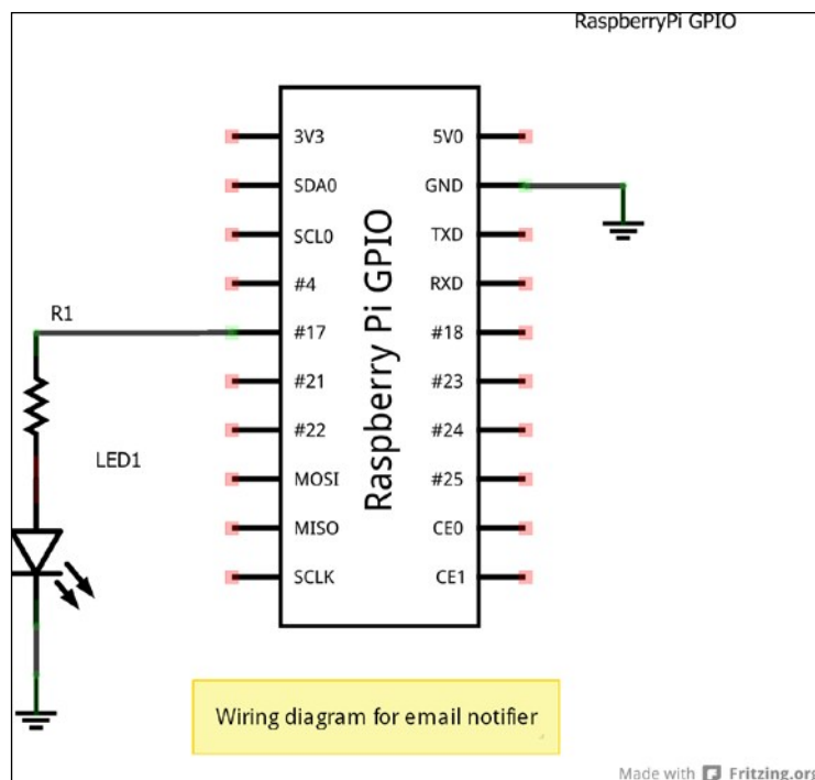
Raspberry Pi email notifier – Schematic created with Fritzing, Raspberry Pi Library
