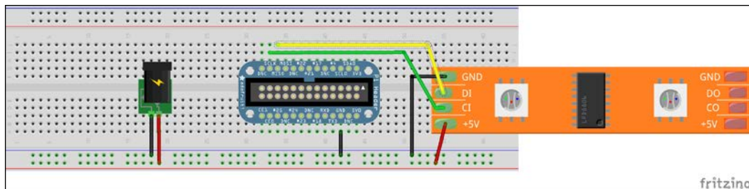
Connecting the RGB LED Strip to the Raspberry Pi using a Pi Cobbler
