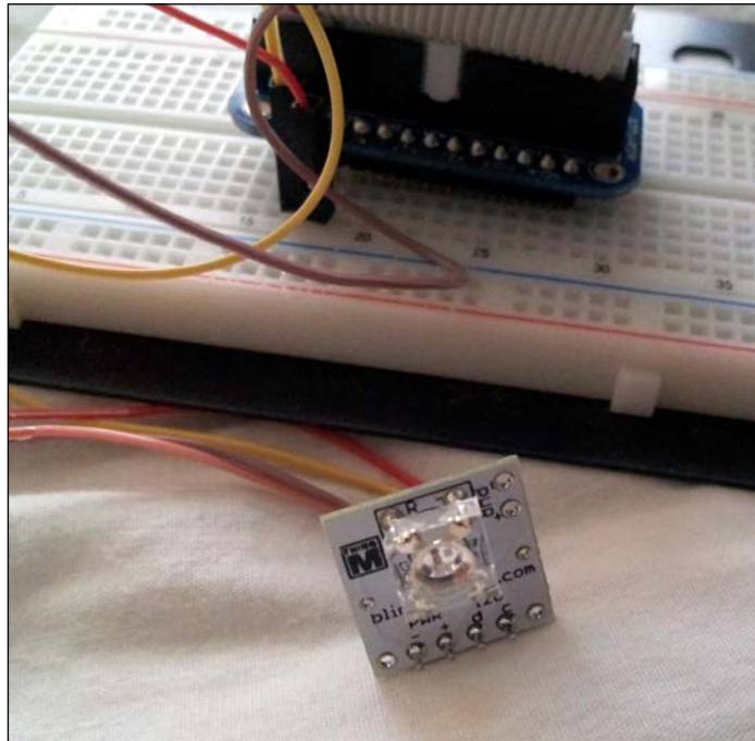
BlinkM connected to the Cobbler
