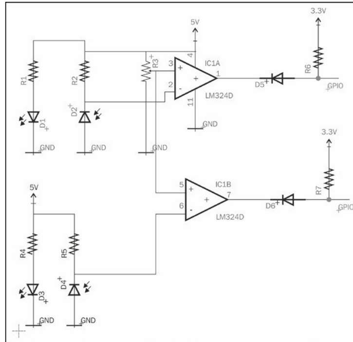
An IR emitter/detector for the line following robot
