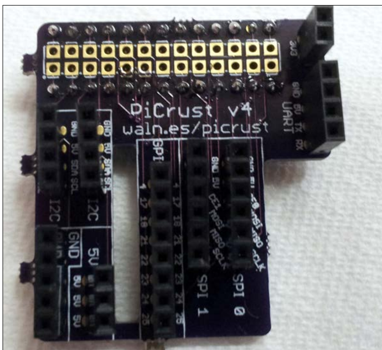
A Pi Crust board
