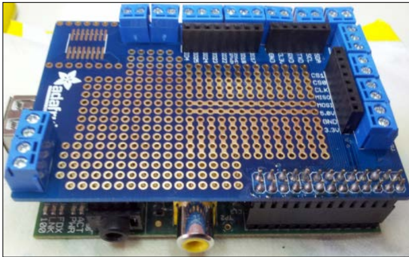
A Pi Plate stacked on the Raspberry Pi
