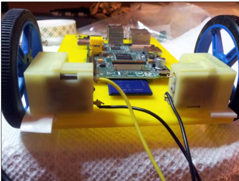
DC motors mounted using double-sided tape
