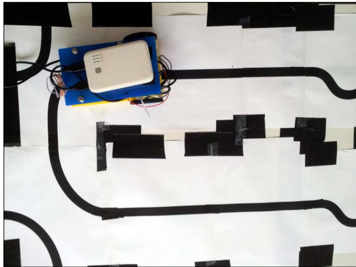
A line following robot on the arena
