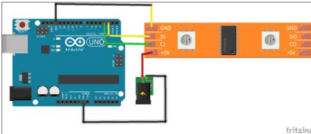
An Arduino connection to the digitally addressable interface
