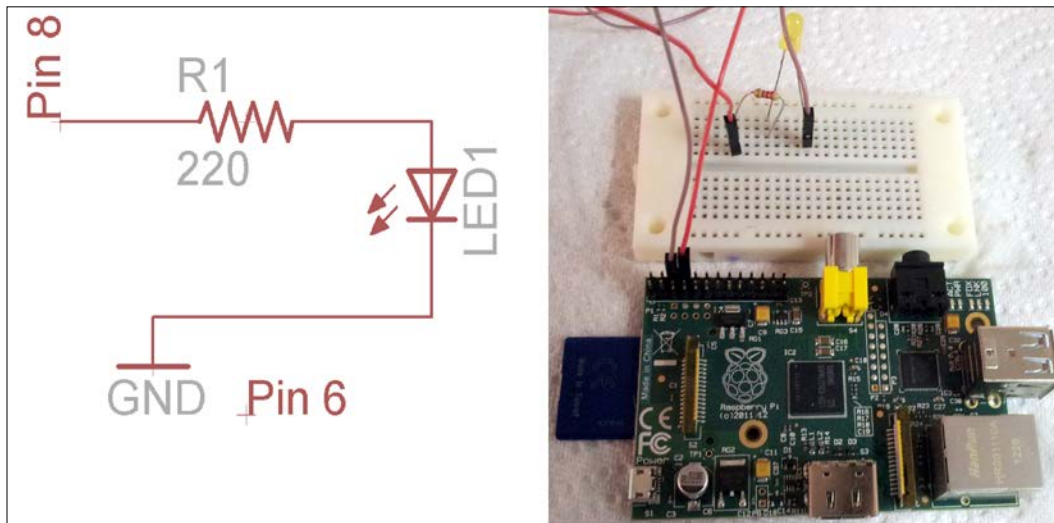
LED blinking circuit
