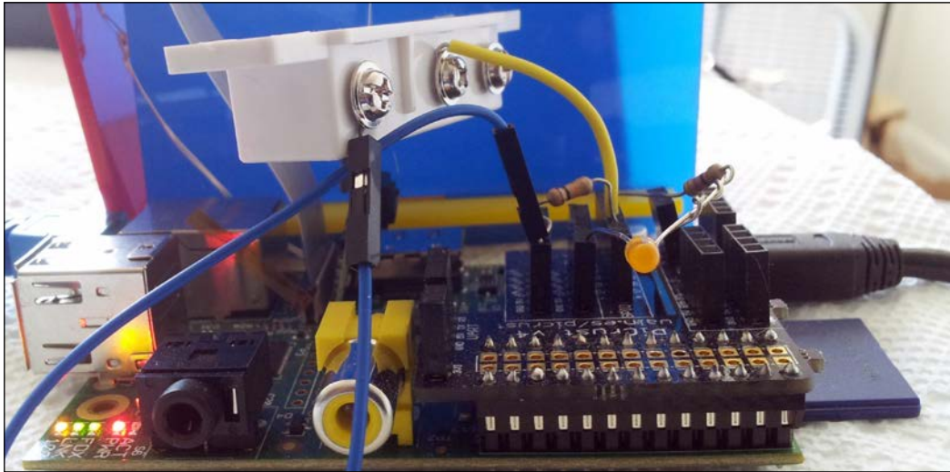
Reed switch interfaced to Raspberry Pi
