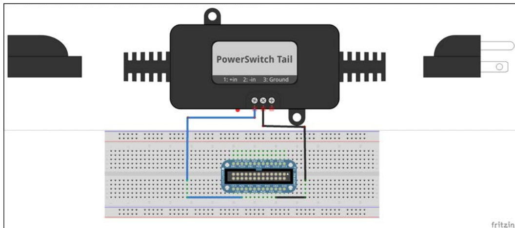
PowerSwitch Tail 2's interface to Raspberry Pi
