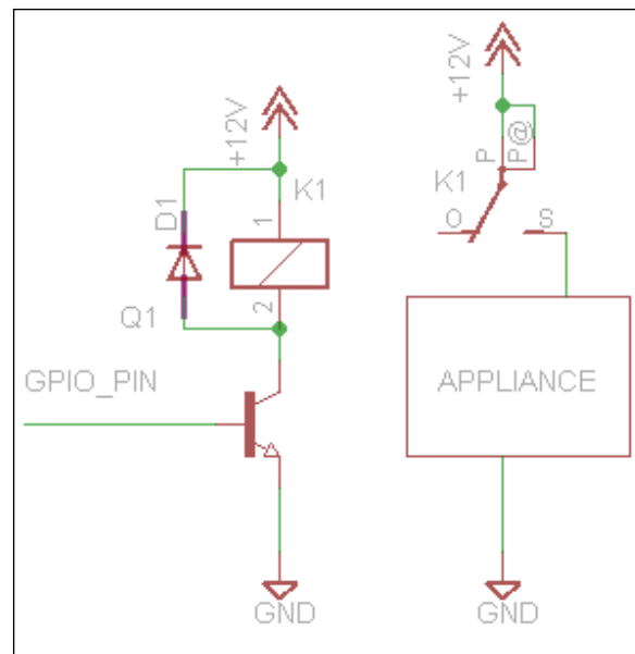
A transistor switching circuit
